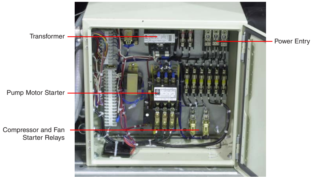
Electrical Cabinet
